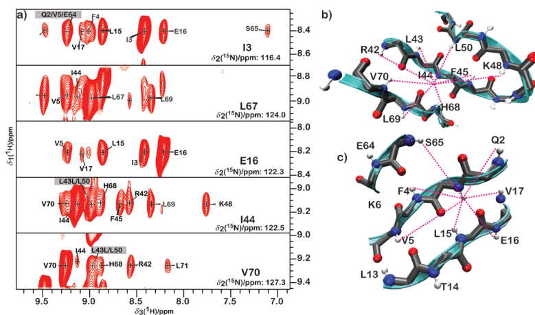
Figure 2. Amide restraints from 3D spectra of backprotonated ( ^2\text{H} , ^{13}\text{C} , ^{15}\text{N} )-ubiquitin. a) Strip plot from a ^1\text{H} -detected 3D ^{15}\text{N} -resolved rotating-frame [ ^1\text{H} , ^1\text{H} ] spin-diffusion experiment. The ambiguous crosspeaks are highlighted by gray boxes around the label; all other labeled crosspeaks are spectrally unambiguous. b, c) Map of the correlations observed in the strip plots in (a) to the structural element from the X-ray structure (PDB code: 3ONS).
