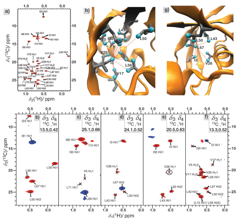
Figure 3. Spectra of ILV-labeled ubiquitin. a) 2D ^1\text{H} - ^{13}\text{C} HSQC spectrum at a MAS frequency of 94.5 kHz and a sample temperature of 20 °C. b–f) 2D planes ( f_1 – f_2 dimensions) of the nonuniformly sampled 4D HSQC-DREAM-HSQC experiment. Positive peaks (diagonal peaks) are depicted in blue while negative peaks (cross-peaks) are depicted in red. 2D planes of b) I61 H \delta 1, c) L69 H \delta 1, d) L67 H \delta 2, e) V26 H \gamma 1, and f) I3 H \delta 1. g, h) Representation of the methyl–methyl correlations observed in the 4D experiments for the L67 \delta 2 and I3 \delta 1 methyl groups by red lines on the X-ray structure. CHD 2 groups are depicted as cyan spheres.
